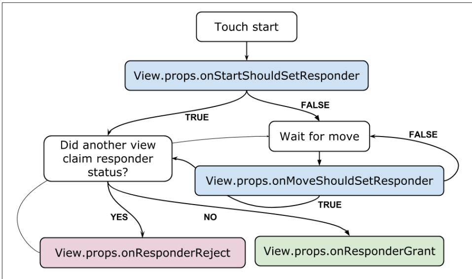
Figure 3-3. Obtaining touch responder status
