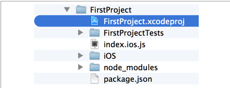
Figure 2-1. File structure in the default project
