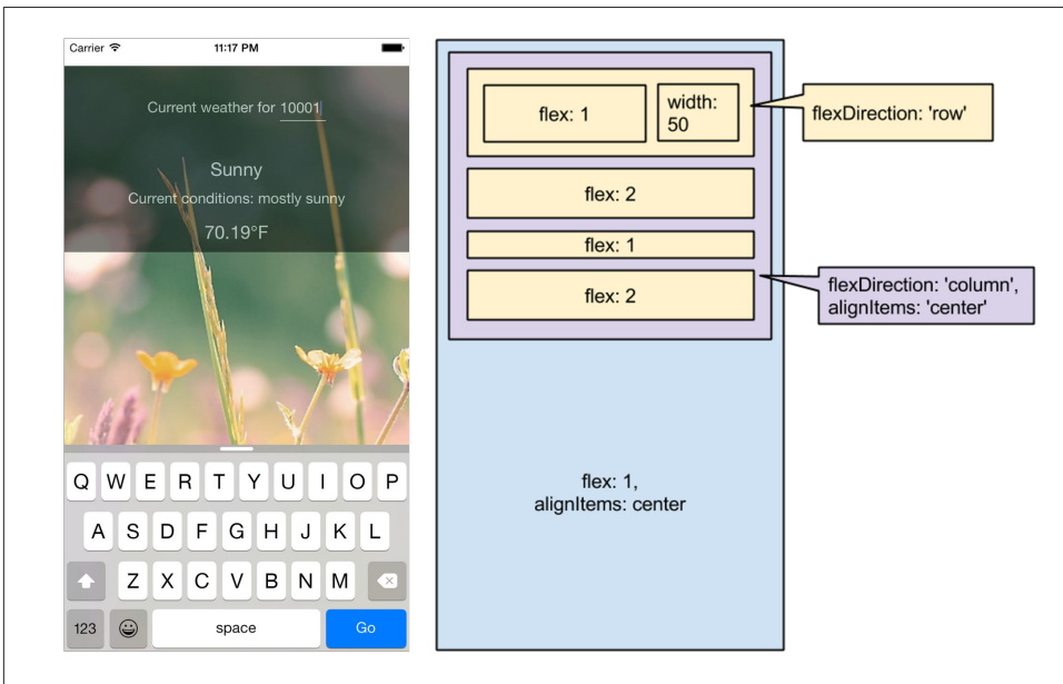
Figure 2-11. Layout of the finished weather application.
