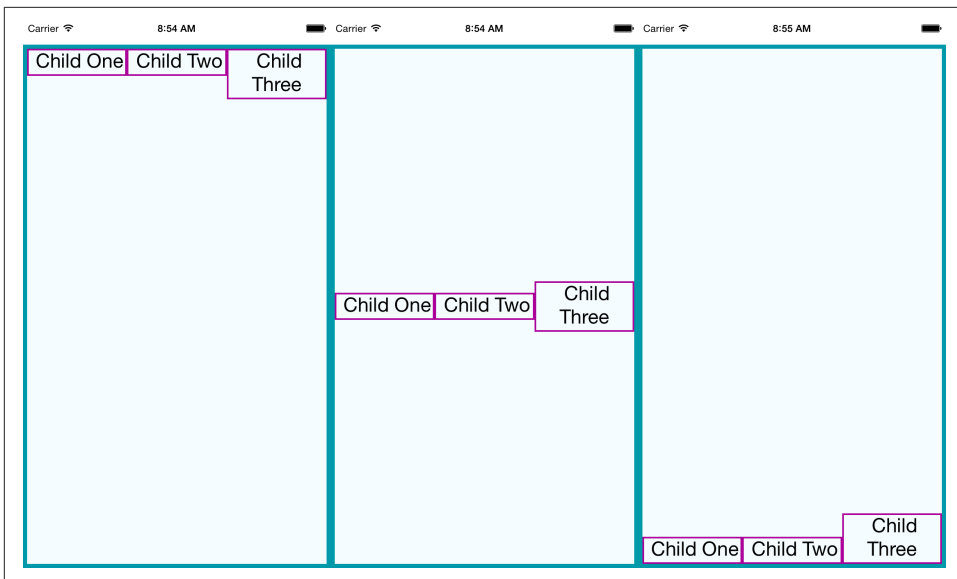
Figure 4-3. Setting alignItems positions children on the cross-axis, which is the axis orthogonal to the flexDirection . Here we see flex-start , center , and flex-end .
