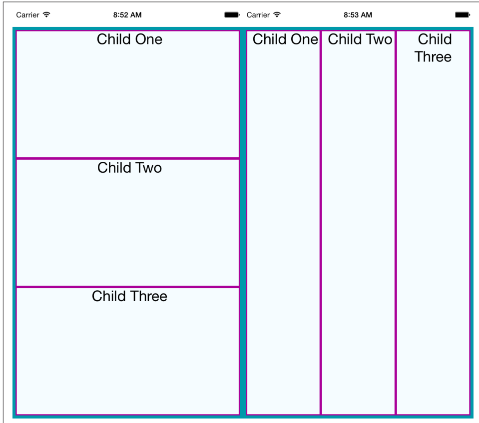
Figure 4-2. Setting basic flex properties, and flexDirection . Left: setting flexDirection to column . Right: setting flexDirection to row .
